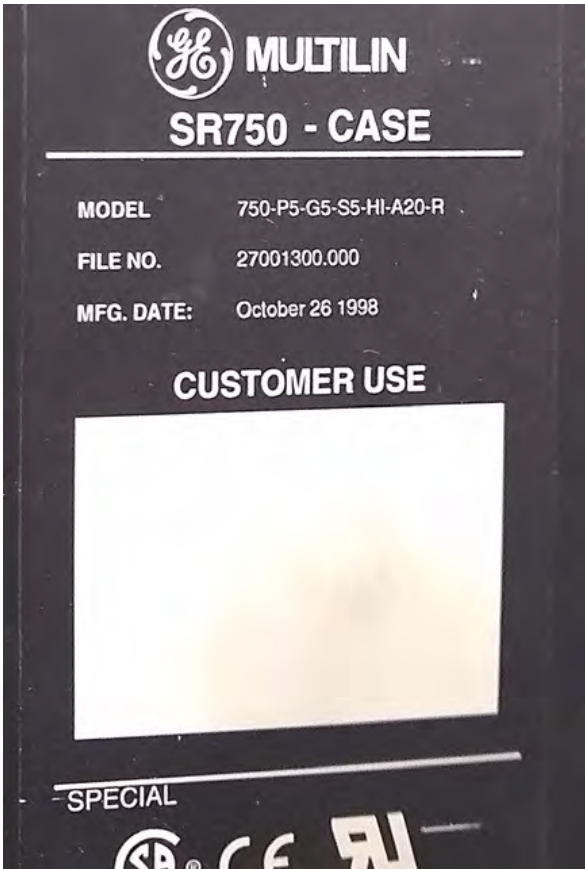
RS01 Feeder CB GE 750 Protection Relay Nameplate
