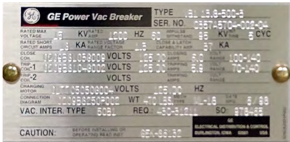
RS02 Feeder CB Nameplate
