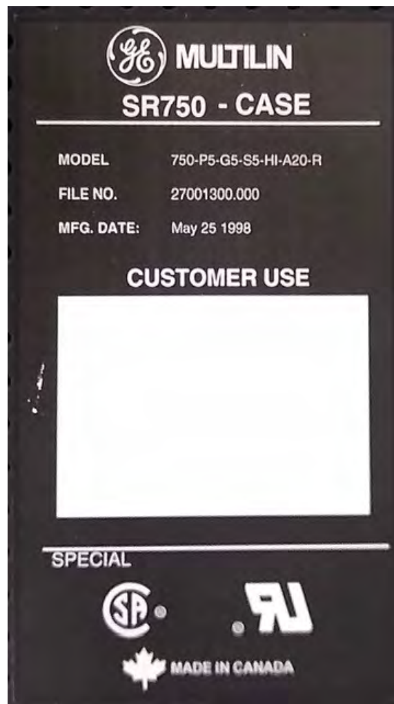
RS02 Feeder CB GE 750 Protection Relay Nameplate
