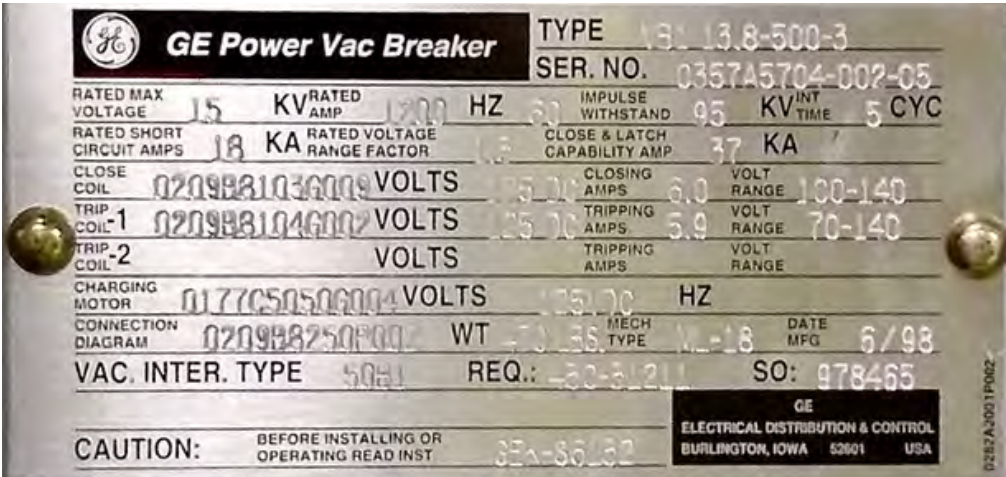
RS01 Feeder CB Nameplate
