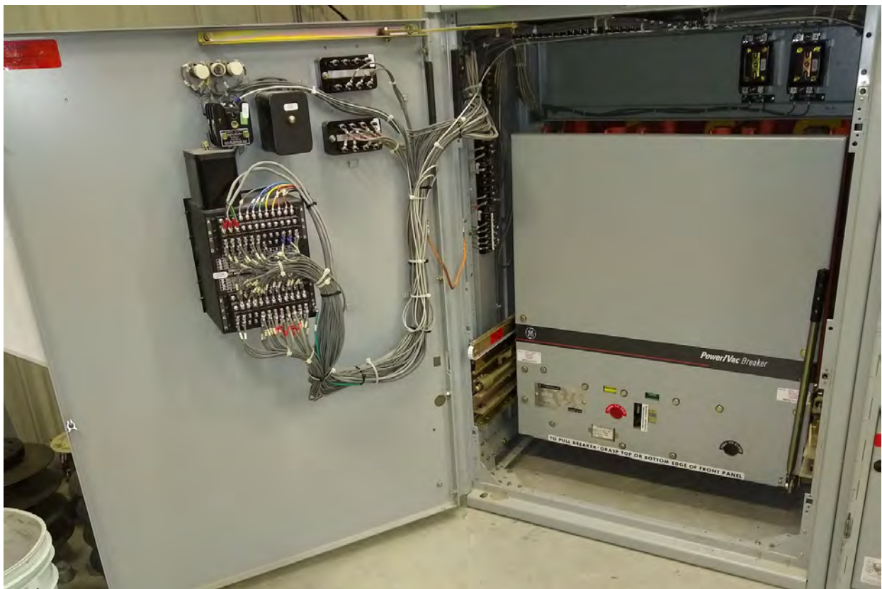
MAIN CB Section Internal View
