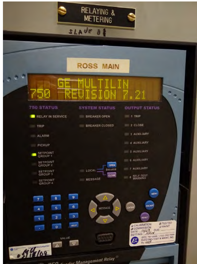
MAIN CB GE 750 Protection Relay Faceplate
