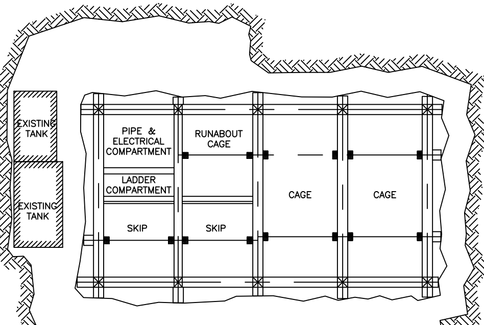
EXISTING YATES 2300 LEVEL SHAFT PLAN
