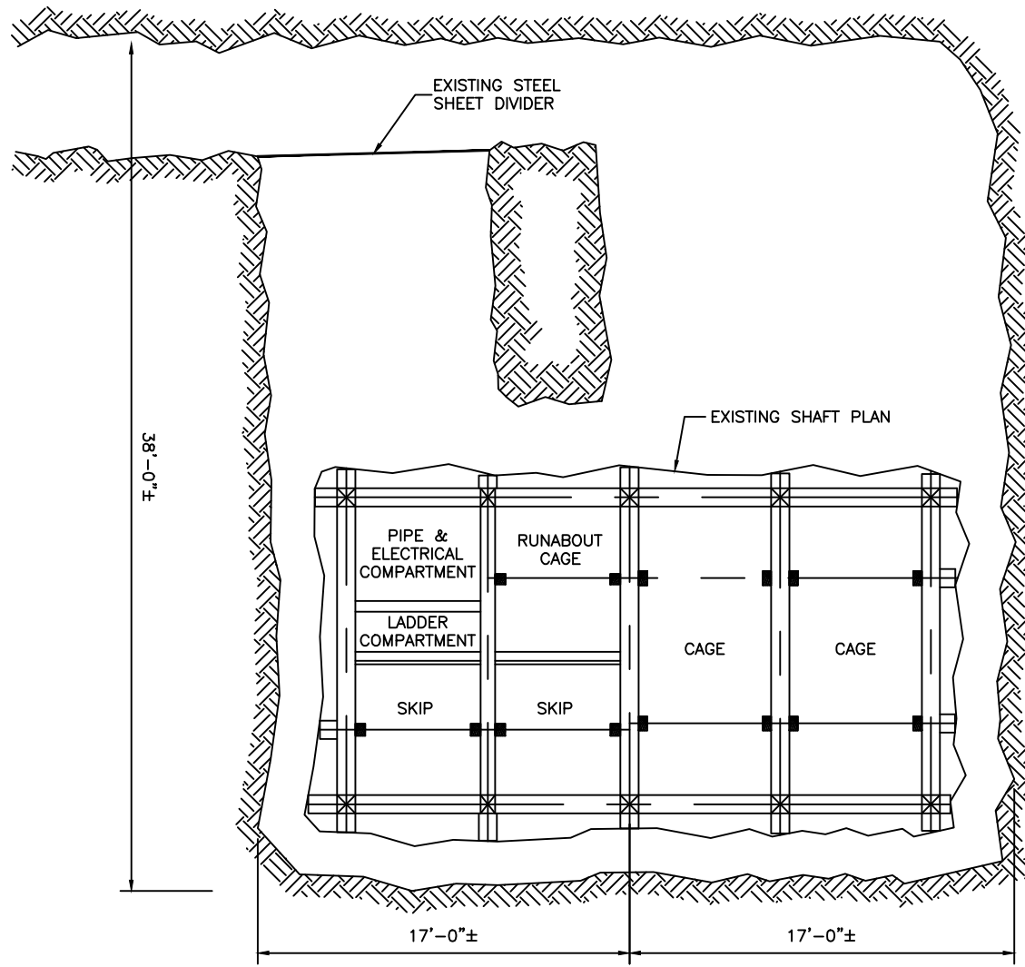
EXISTING YATES 800 LEVEL SHAFT PLAN
