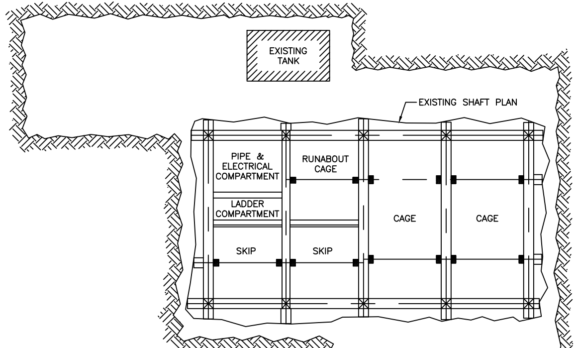
EXISTING YATES 1100 LEVEL STATION PLAN
