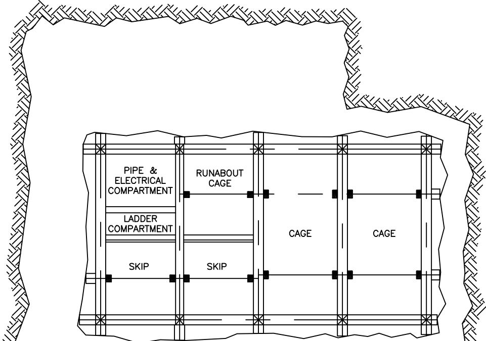
EXISTING YATES 2900 LEVEL SHAFT PLAN
