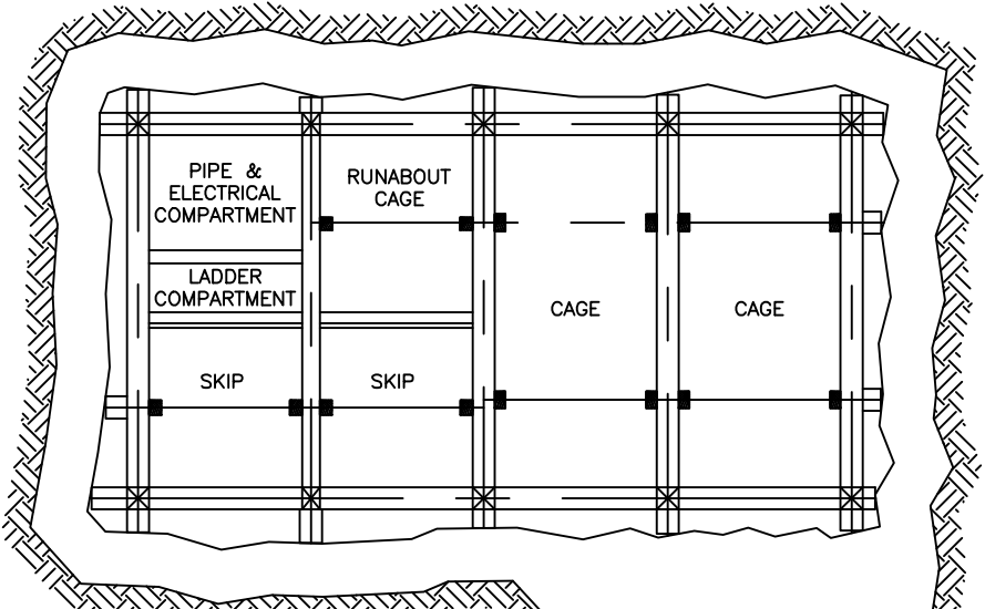
EXISTING YATES 1850 LEVEL SHAFT PLAN
