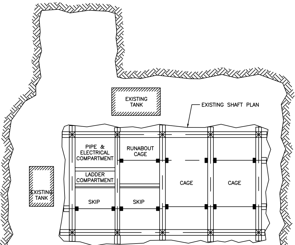
EXISTING YATES 1700 LEVEL SHAFT PLAN
